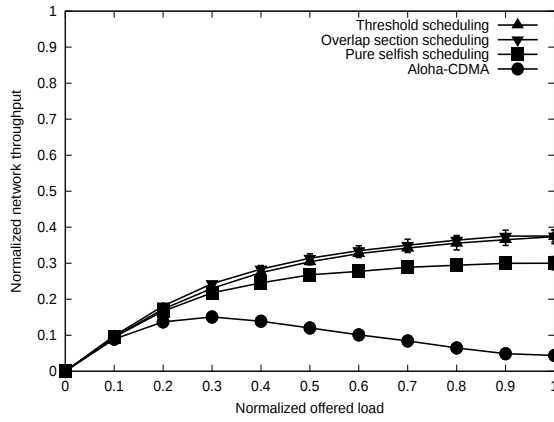
Fig. 7. Comparison of the performance of the transmission scheduling algorithms based on simulation. The traffic model is Poisson arrivals with exponentially distributed packet lengths. The codeset is (10, 3, 3) and codewords are chosen uniform randomly. For the threshold scheduling algorithm, the threshold parameter was set to 0.5
